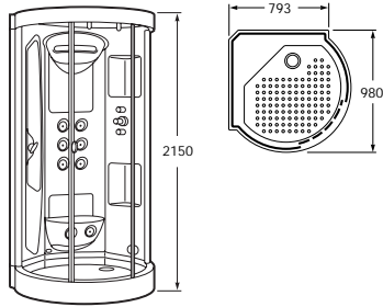
Aquatech Basic Vapor 900
